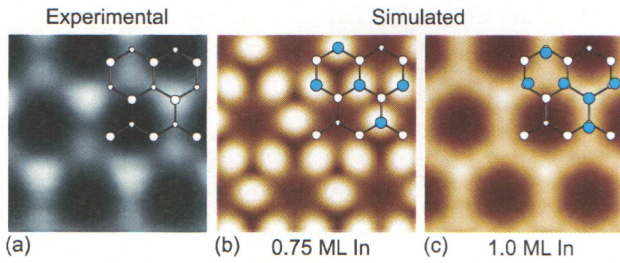
FIG. 2. (Color online) (a) Filled-state (+1.3 V) experimental STM image of the In/Si(111) 2\times 2 surface compared with the simulated STM images (+1.0 V) for (b) 0.75-ML model and (c) 1.0-ML model. To tie the STM images to the surface structure, the schematic of the Si(111) surface structure is superposed on the experimental STM image and model structures on the corresponding simulated STM images. In atoms are shown by blue circles, Si atoms are shown by open circles, the larger for on-top Si atoms in T_1 sites, the smaller for the Si atoms in the T_4 site.
